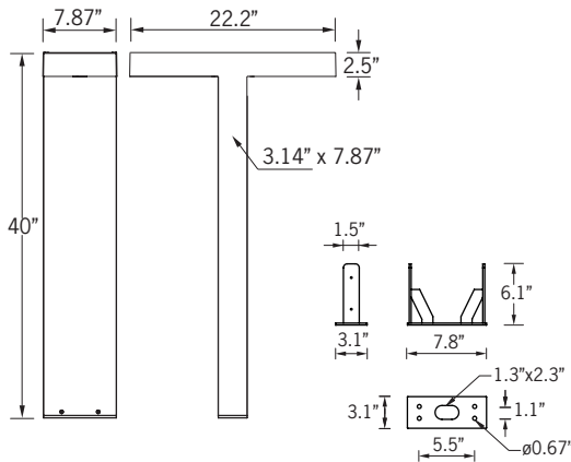
Mounting Detail
